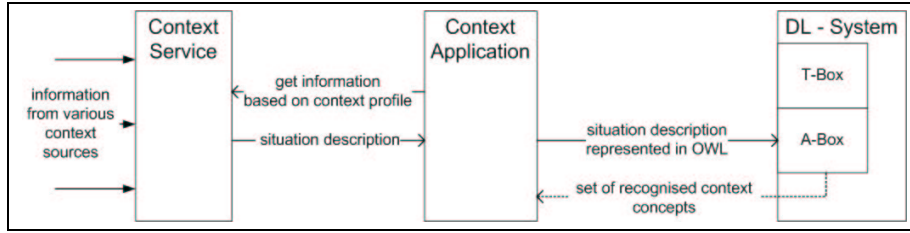
Figure 1. Main components of our context framework.
