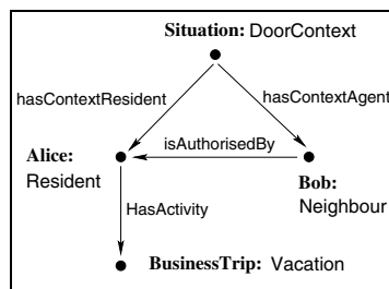
Figure 3. An ABox fragment.
