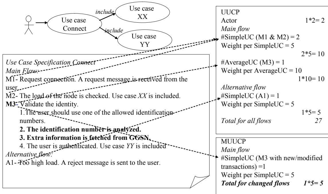
Figure 2. Example of counting UUCP and MUUCP for a use case called Connect
