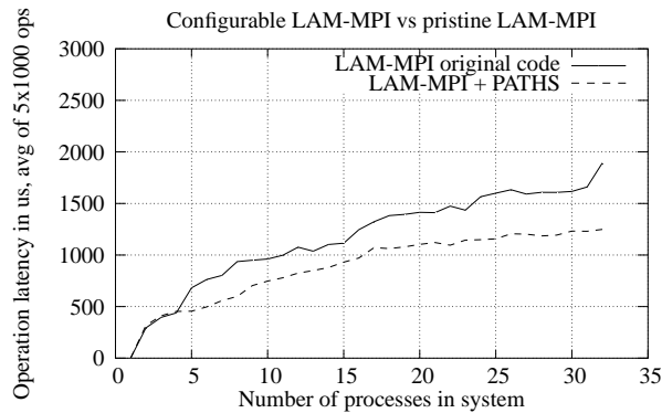
Figure 7: Allreduce, 2-way cluster.
