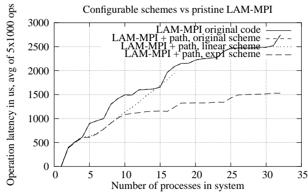
Figure 5: Allreduce, 4-way cluster
