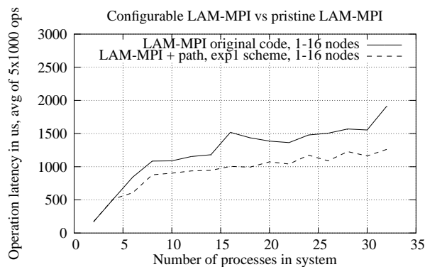
Figure 8: Allreduce, 2-way cluster, scaling the number of nodes from 1 to 16. Each node added adds two new processes in the experiment.
