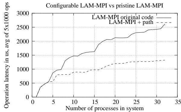
Figure 6: Allreduce, 8-way cluster
