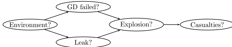
Figure 1: An example BN describing a gas leak scenario. Only the qualitative part of the BN is shown.
