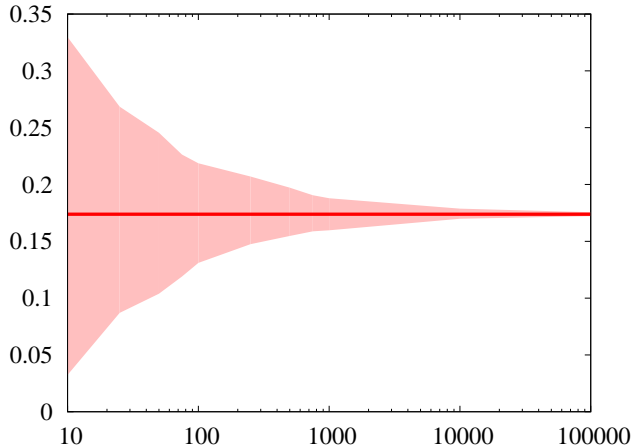
Figure 10: Uncertainty of the estimate of P(\mathbf{T} = \mathbf{1}) as a function of the number of samples is displayed as the 5% and 95% quantiles (1000 repetitions).
