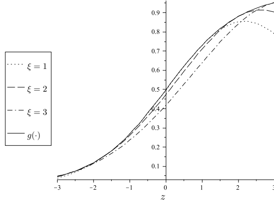
Figure 8: The solid line shows the logistic function with \mathbf{w} = [1, 1]^T and b = 0 (as in our example). The three other functions correspond to the variational approximations defined by \xi = 1 , \xi = 2 , and \xi = 3 , respectively; \xi is chosen so to maximize the expected lower bound of the data-complete marginal likelihood, hence it also depends on the prior distribution for the explanatory variables.
