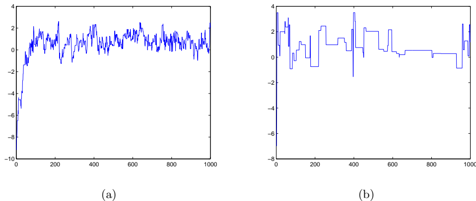
Figure 11: The figures show the samples for Z_1 using the proposals distributions N(\mathbf{z}_t, \frac{1}{2}\mathbf{I}) and N(\mathbf{z}_t, 5\mathbf{I}) , respectively.
