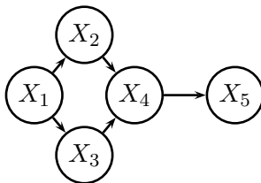
Figure 2: An example of Bayesian network.
