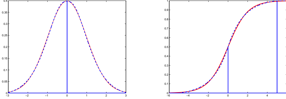
Figure 6: Results of the MTE approximation in our running example: The approximation to each distribution is dashed, the true underlying density (Normal in the left panel and the logistic in the right) is given with solid line.
