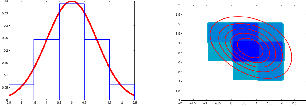
Figure 5: Results of discretization in our running example. The left pane gives the approximation of the Gaussian distribution, whereas the right panel shows the approximation of f(z_1, z_2 | \mathbf{T} = \mathbf{1}) together with the exact results (obtained by numerical integration). Note the poor approximation to the joint posterior distribution, particularly in the tail of the distribution.
