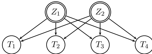
Figure 4: A model for the analysis of human reliability. A subject’s ability to perform four different tasks T_1, \dots, T_4 is influenced by the two explanatory variables Z_1 and Z_2 . The explanatory variables are drawn with double-line to signify that these variables are continuous.
