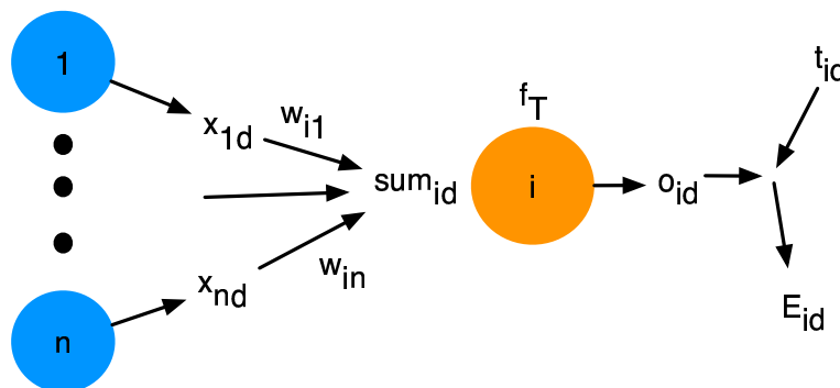
Figure 1: Simple perceptron with n weighted input lines
