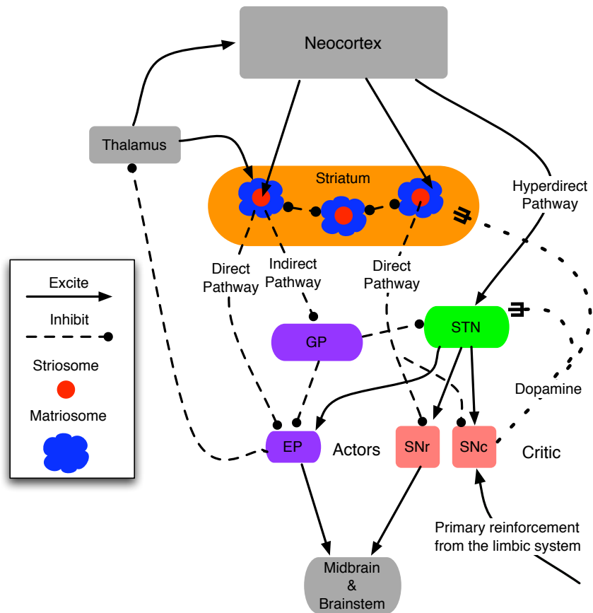
Figure 10: Functional topology of the basal ganglia and their main inputs, derived from text and diagrams in [25, 26, 40, 21]. The actor denotes the direct outputs of the BG: EP and SNr, while the critic consists of the diffuse neuromodulatory output from SNc. Matriosomes are primarily gateways to the actor circuit, while striosomes have direct-pathway links to both actors and critics.
