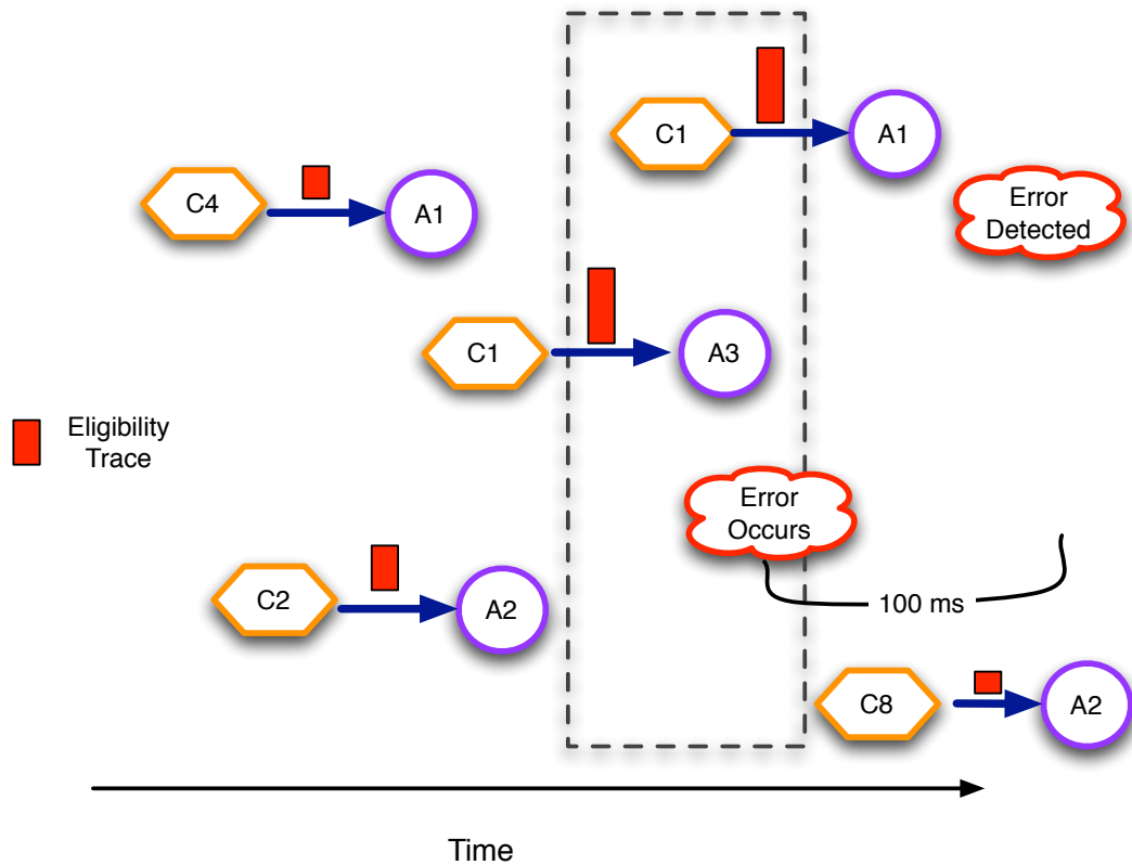
Figure 7: Cerebellar eligibility traces, drawn as rectangles on the condition-action arcs, with taller rectangles denoting higher eligibility. Synapses are most eligible for modification approximately 100 milliseconds after they transmit an action potential.
