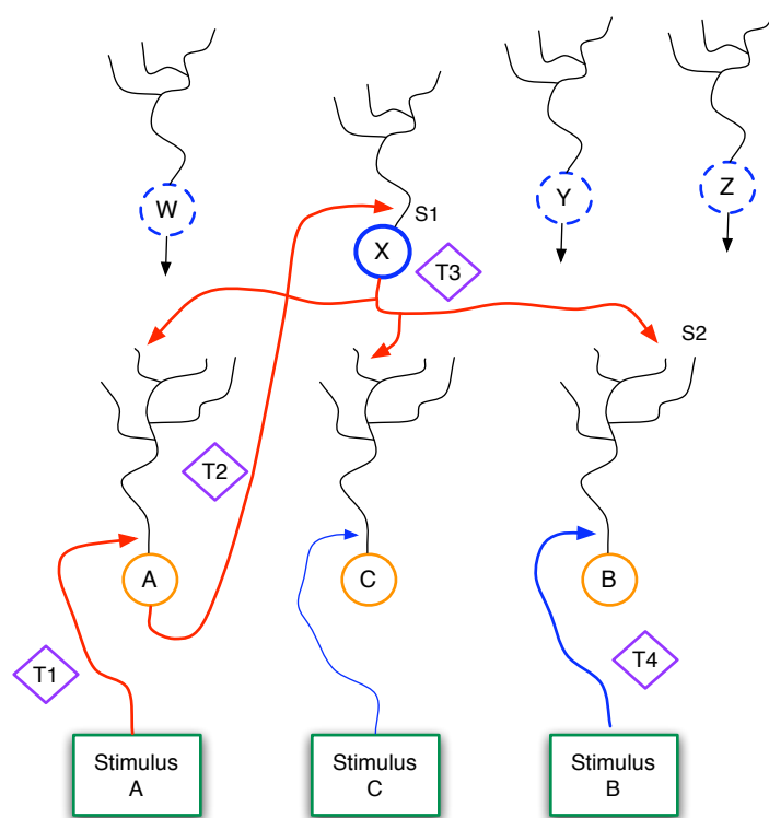
Figure 13: The Generic Declarative Prediction Network (GDPN). Neurons A, B and C serve as low-level detectors for stimuli A, B and C, while W-Z represent neurons at a higher level. Only the axonal projections from X are shown, though W, Y and Z have similar links to the lower level. The T1 - T4 diamonds represent time steps, while S1 and S2 denote important synapses, as further discussed in the text.
