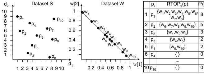
Figure 2: Most influential data objects.
