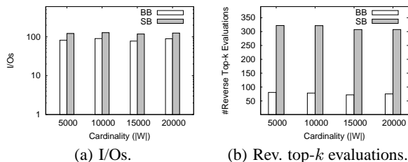
Figure 10: BB vs. SB for UN dataset and varying |W| .
