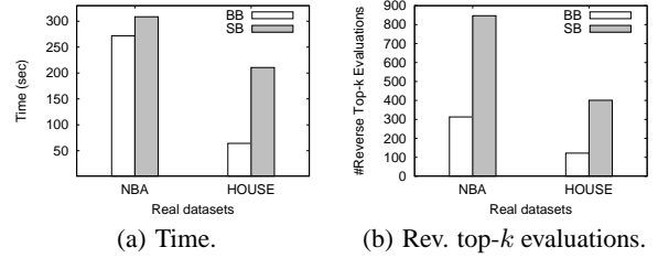
Figure 15: BB vs. SB for real data.
