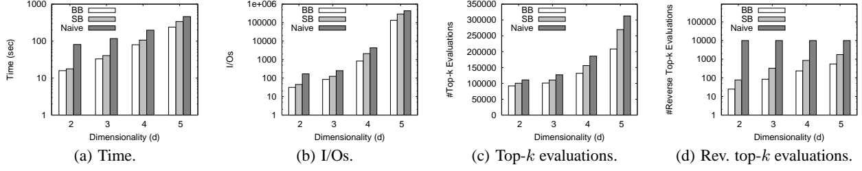
Figure 5: Comparative performance of all algorithms for UN dataset and varying dimensionality ( d ).
