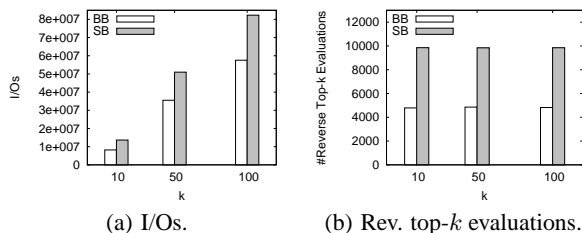
Figure 11: BB vs. SB for AC dataset and varying k .
