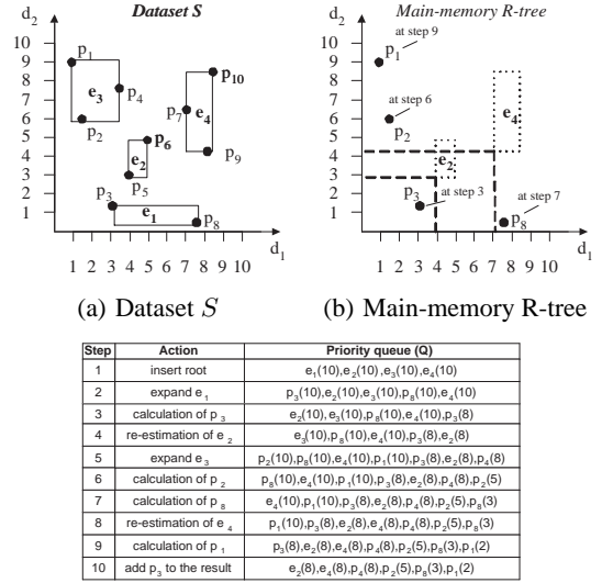
(c) Contents of priority queue Q Figure 4: Example of execution of algorithm BB .
