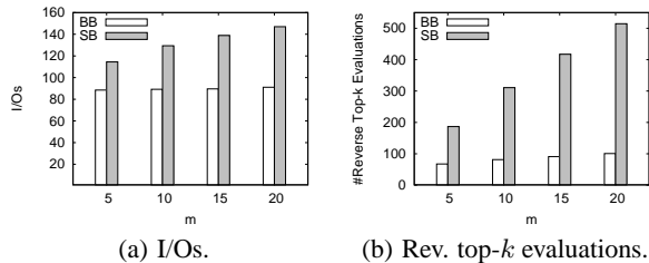
Figure 12: BB vs. SB for UN dataset and varying m .
