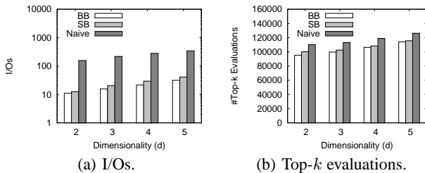
Figure 13: All algorithms for CO dataset and varying d .
