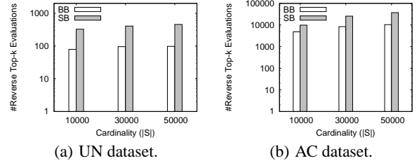
Figure 8: BB vs. SB for varying |S| .
