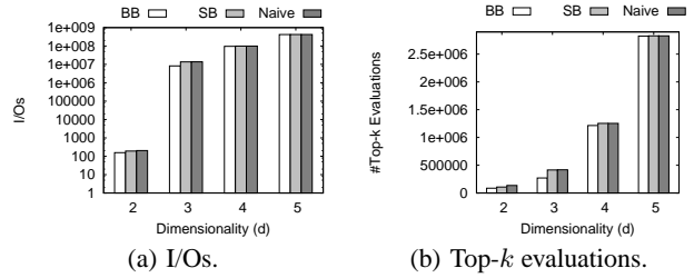
Figure 14: All algorithms for AC dataset and varying d .
