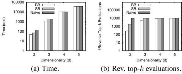
Figure 7: All algorithms for AC dataset and varying d .
