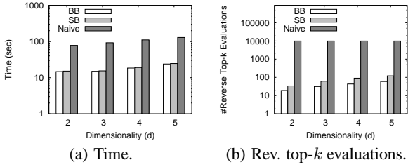
Figure 6: All algorithms for CO dataset and varying d .
