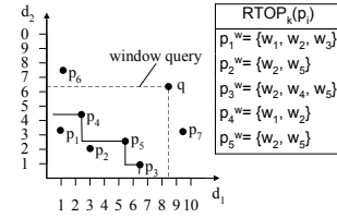
Figure 3: Upper bound of influence score of q .
