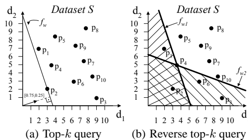
Figure 1: Top- k and reverse top- k query.
