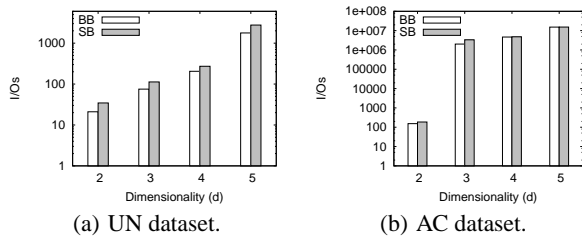
Figure 9: BB vs. SB for clustered W .
